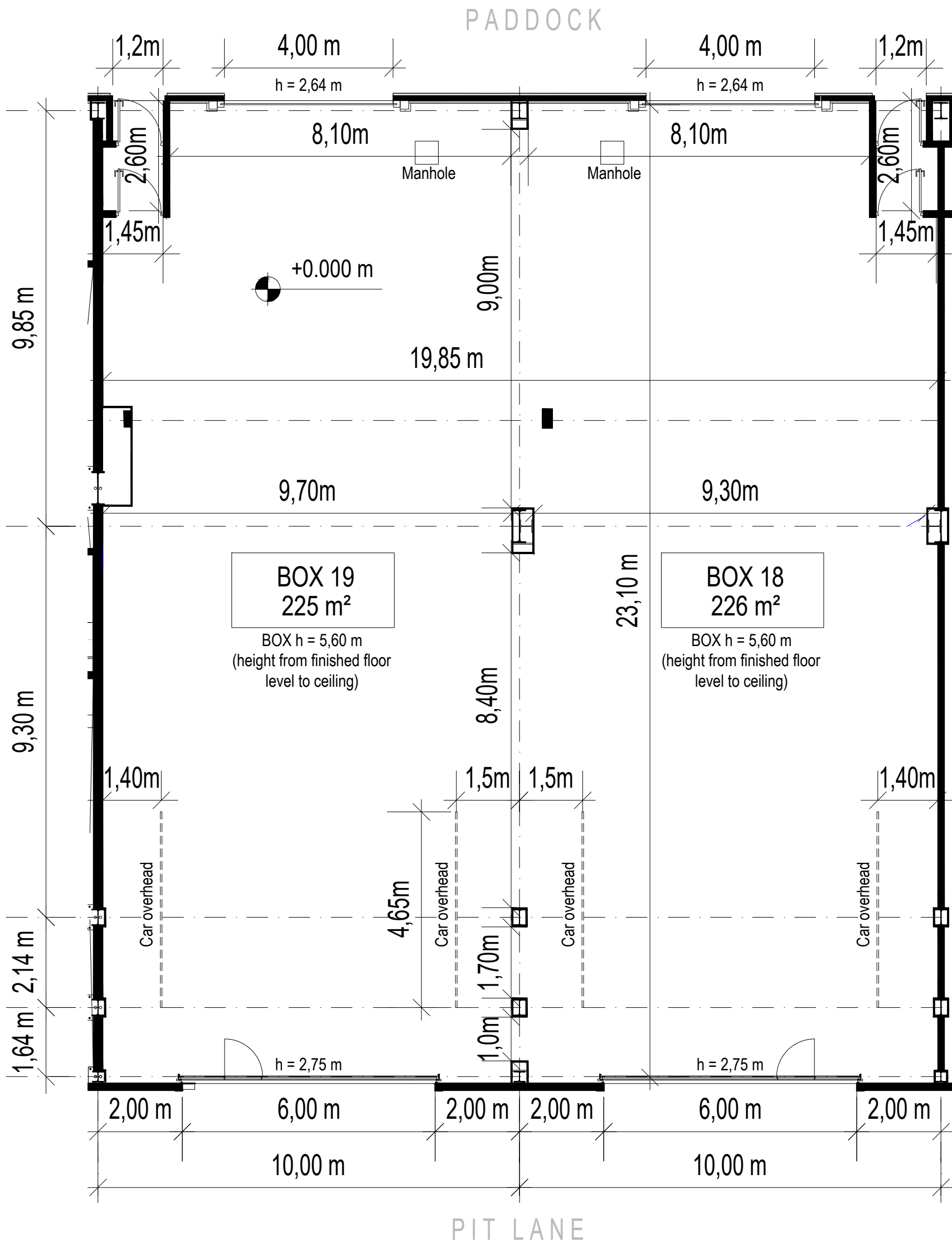
Pit Building - Permanent Building A GROUND FLOOR
